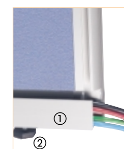
① Cable holder ② Stabilizer feet, adjustable through 20 mm.
